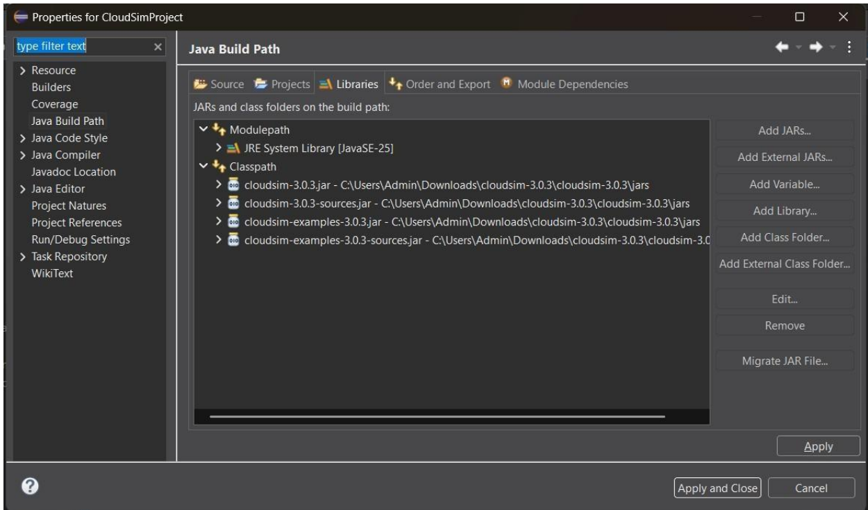
Fig 1.3: CloudSimProject properties
